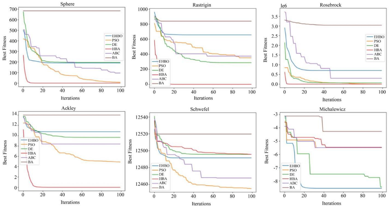
Fig. 1 Convergence curves for Benchmark functions
