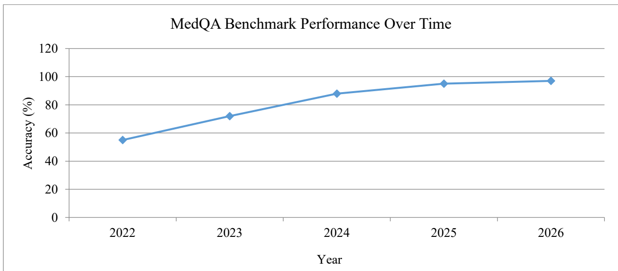
Fig. 2 Accuracy Evaluation
