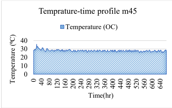
Fig. 7 Temperature-Time Profile for a) M35 b) M40 c) M45 Concrete Grade
